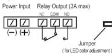
Fig.1 – Connections
